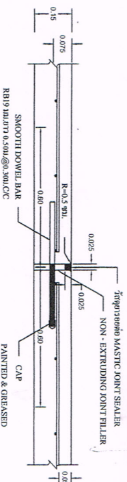
APPLICATION EXPANSION JOINT
